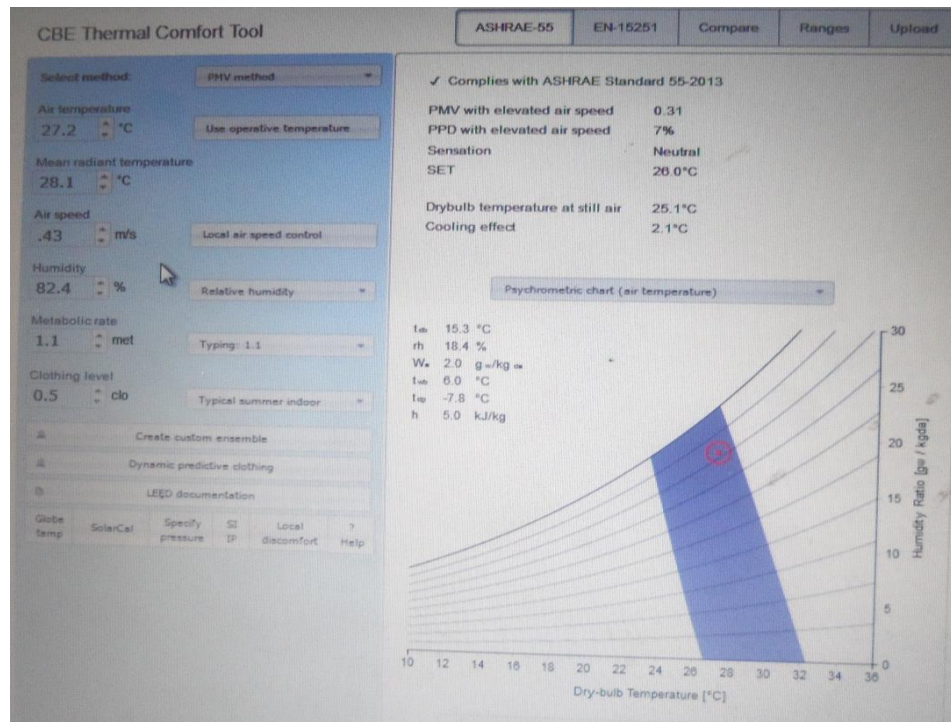
Fig. 6: Effect of air speed on thermal comfort of Case Study 2B building at assumed air velocity of 0.43m/s
